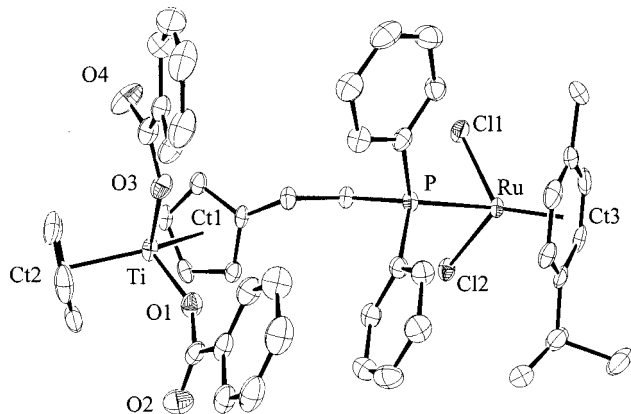
Figure 1. Molecular structure of complex 8 . The \text{CH}_2\text{Cl}_2 solvate molecule and the benzoic acid have been omitted for clarity. Selected bond lengths [Å] and angles [°]: Ti–Ct1 2.049(3), Ti–Ct2 2.054(4), Ti–O1 1.947(2), Ti–O3 1.956(2), Ru–Ct3 1.707(3), Ru–P 2.3516(8), Ru–Cl1 2.4182(9), Ru–Cl2 2.4211(8); Ct1–Ti–Ct2 132.4(2), O1–Ti–O3 90.8(1), Ct3–Ru–P 130.6(1), Ct3–Ru–Cl1 127.3(1), Ct3–Ru–Cl2 124.7(1), P–Ru–Cl1 85.25(3), P–Ru–Cl2 85.89(3), Cl(1)–Ru–Cl(2), 89.16(3) Ti–O(1)–C(35) 152.9(2), Ti–O3–C42 142.4(2).
