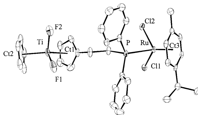
Figure 2. Molecular structure of complex 10 . The \text{CDCl}_3 solvate molecules have been omitted for clarity. Selected bond lengths [Å] and angles [°] [data in square brackets correspond to the second independent molecule]: Ti–Ct1 2.050(5) [2.055(5)], Ti–Ct2 2.065(5) [2.056(5)], Ti–F1 1.891(3) [1.905(4)], Ti–F2 1.937(3) [1.896(4)], Ru–Ct3 1.707(4) [1.709(4)], Ru–P 2.347(1) [2.344(1)], Ru–Cl1 2.4180(12) [2.4093(13)], Ru–Cl2 2.4126(13) [2.4200(11)]; Ct1–Ti–Ct2 132.6(2) [136.2(2)], F1–Ti–F2 93.70(14) [95.7(2)], Ct3–Ru–P 131.0(1) [130.6(1)], Ct3–Ru–Cl1 126.1(1) [126.1(1)], Ct3–Ru–Cl2 127.7(1) [127.3(1)], P–Ru–Cl1 84.35(3) [83.47(3)], P–Ru–Cl2 86.92(4) [86.74(4)], Cl1–Ru–Cl2 86.80(4) [86.84(4)].
