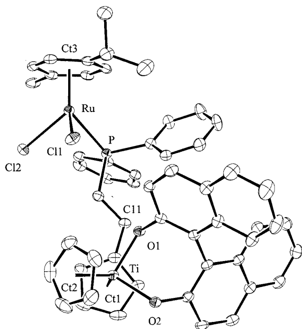
Figure 3. Molecular structure of complex rac -12. Only one enantiomer is shown for clarity. The free binaphthol molecule and the \text{CH}_2\text{Cl}_2 solvate molecules are also not shown. Selected bond lengths [Å] and angles [°]: Ti–Ct1 2.099(3), Ti–Ct2 2.088(4), Ti–O1 1.915(2), Ti–O2 1.981(2), Ru–Ct3 1.703(3), Ru–P 2.3442(8), Ru–C11 2.4210(7), Ru–Cl2 2.4157(8), Ct1–Ti–Ct2 130.48(13), O1–Ti–O2 91.96(9), Ct3–Ru–P 130.95(9), Ct3–Ru–C11 126.04(9), Ct3–Ru–Cl2 126.42(9), P–Ru–C11 84.97(3), P–Ru–Cl2 86.80(3), C11–Ru–Cl2 87.22(3).
